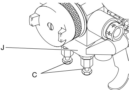
FIG. 11 Manual Valves
